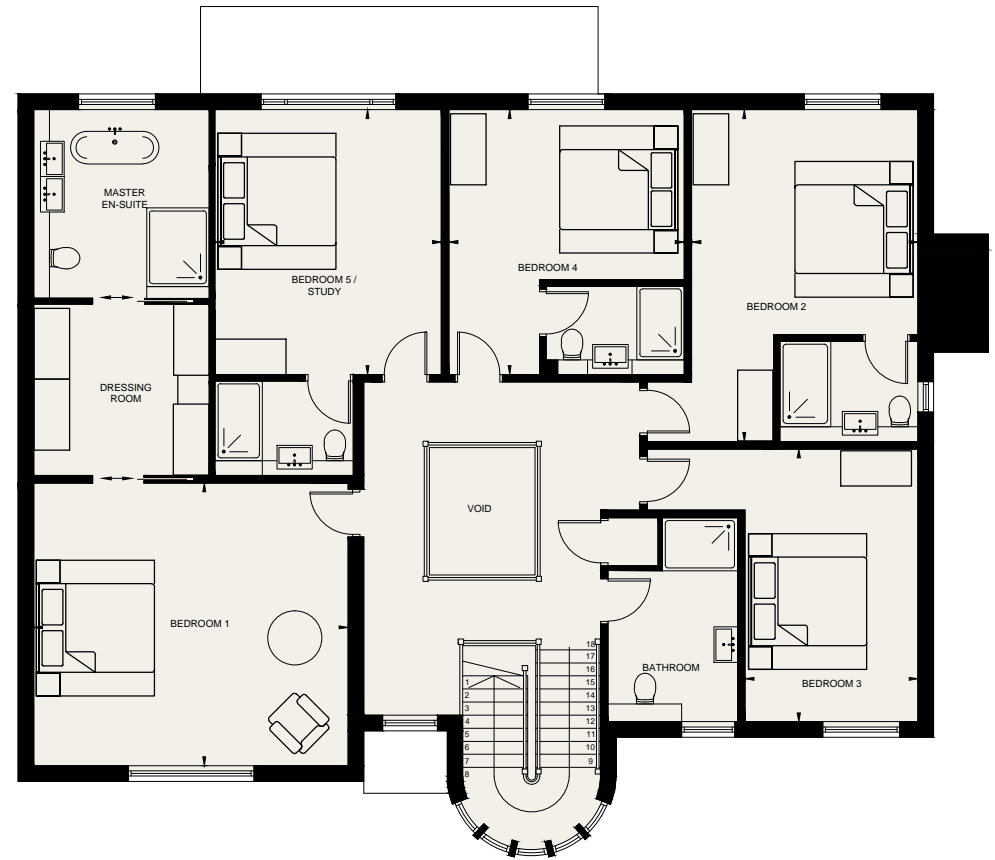
FIRST FLOOR
